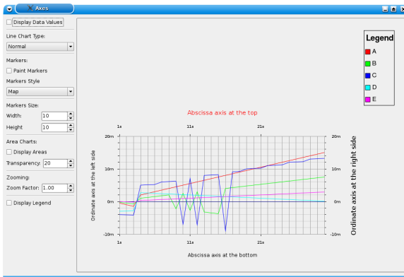
Figure 9.1. /examples/Axis/Parameters
