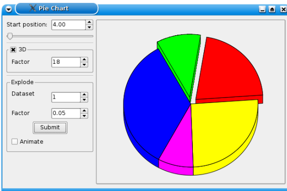
Figure 9.9. /examples/Pie/Advanced
