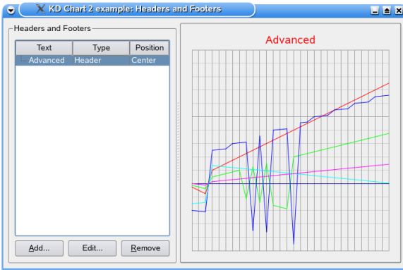
Figure 9.4. /examples/HeadersFooters/HeadersFooters/Advanced
