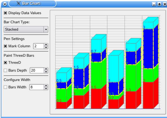
Figure 9.3. /examples/Bars/Advanced
